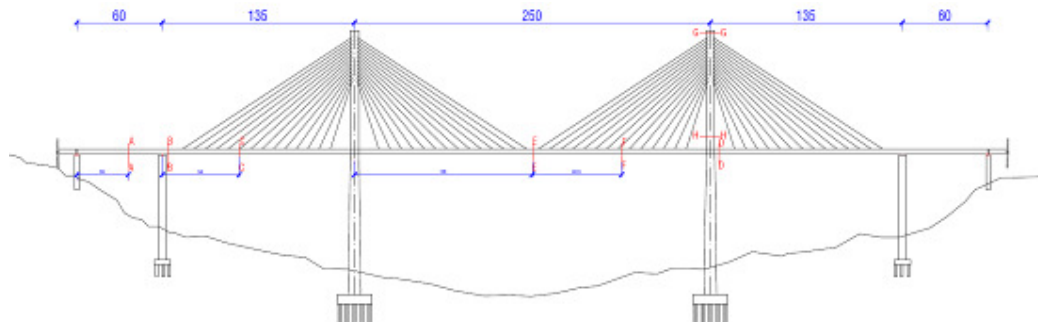
Fig.6 The test section layout diagram(unit: m)
