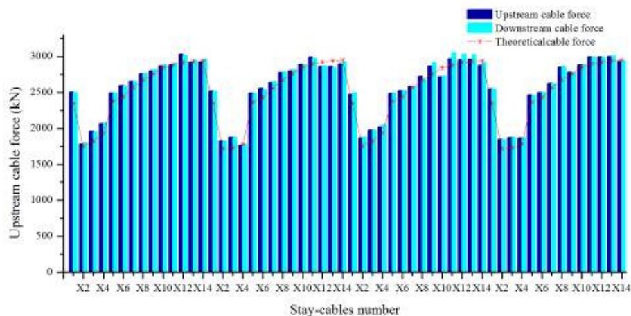
Fig.4 stay cable force distribution map
