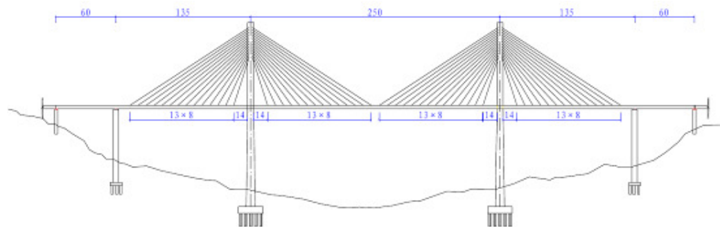
Fig.1 Cable-stayed bridge elevation layout(unit: m)
