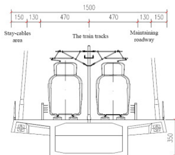
Fig.2 Cable-stayed bridge cross section diagram(unit: cm)
