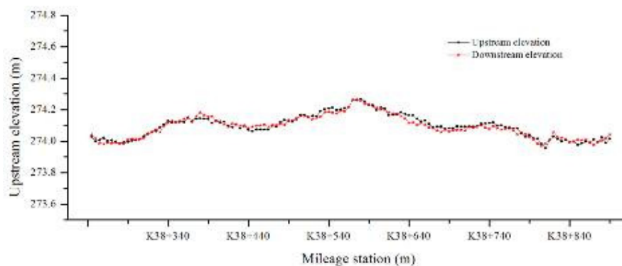
Fig.3 the measured line shape of the girder
