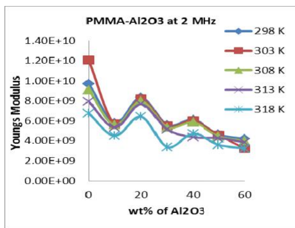
Fig. 6 variation of youngs modulus \text{Al}_2\text{O}_3 conc.
