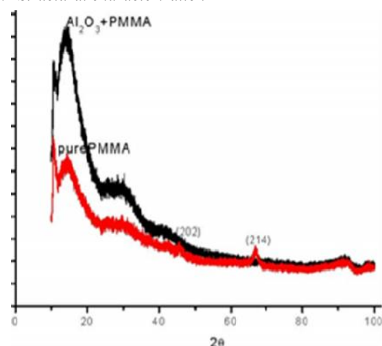
Fig.1 XRD of PMMA and PMMA/ \text{Al}_2\text{O}_3
