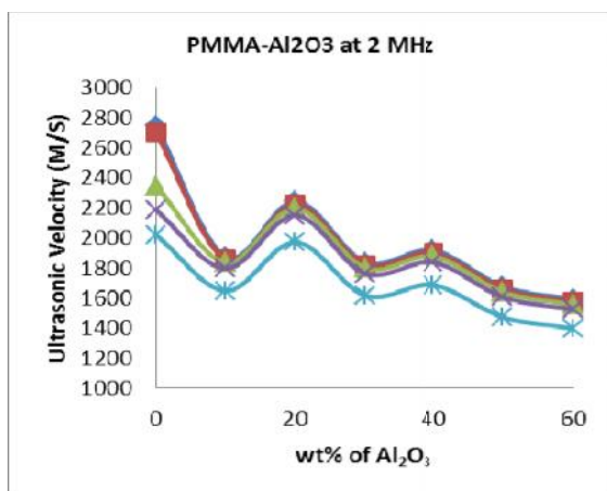
Fig. 3 Variation of ultrasonic velocity at 2MHz
