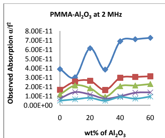
Fig. 4 Variation of Observed absorption at 2MHz
