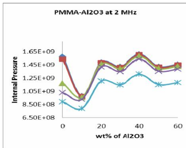
Fig. 5 Variation of Internal Pressure with \text{Al}_2\text{O}_3 conc.
