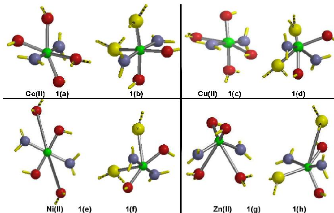
Figure 1: Optimized M(II) skeleton complexes
