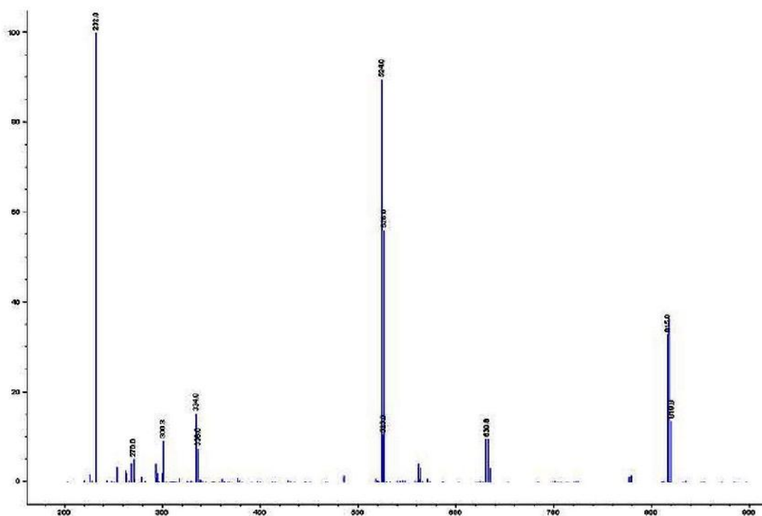
The mass spectrum of the studied Cu(II) Complex
