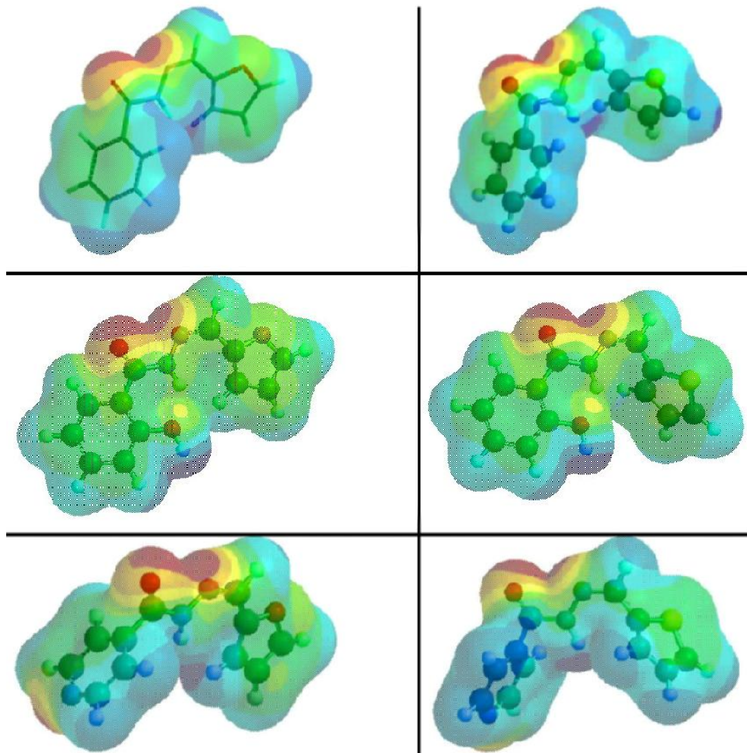
Figure 2: Computed electrostatic potential on the molecular surface of complexes (1,7,14,21) optimized at PM6. The potential ranges according to the color code: red (most negative) < orange < yellow < green < blue (most positive).
