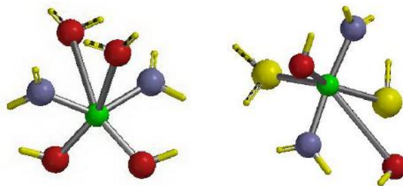
Figure 3: Optimized Mn(II) skeleton complexes
