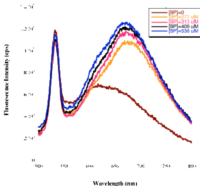
Figure 4 – Fluorescence spectra for [13] using 475 nm excitation for [\text{BP}] = 0 and 277, 313, 409, 536 \mu\text{M} BP. Note: the sharp peak at 530 nm is the Raman line of water, indicating how weak the fluorescence signal is for [13] . The area from 500 to 800 nm under each spectrum was determined (F) and the increase for each BP concentration determined ( \Delta F ). A plot of \Delta F vs. \Delta F/[\text{BP}] yielded a straight line with slope of -(1/K_b) , 8 thus determining K_b = 5 \times 10^3 .
