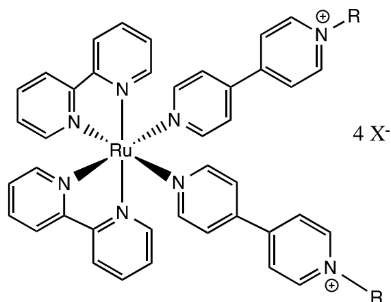
Figure 1 - General structure of the bis(2,2'-bipyridyl) octahedral ruthenium(II) species under consideration in the current report. Additional compounds of interest have (phen) bidentate ligands in place of the bipyridyl (bpy) ligands.
