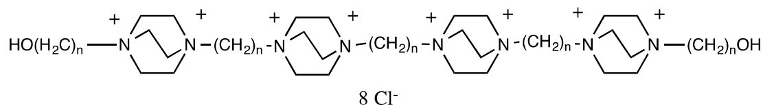
Figure 3 - General structure of "polycationic strings" - Cationic sites are located regularly along a flexible chain and thereby capable of interacting electrostatically with the (anionic) major groove of double stranded DNA.
