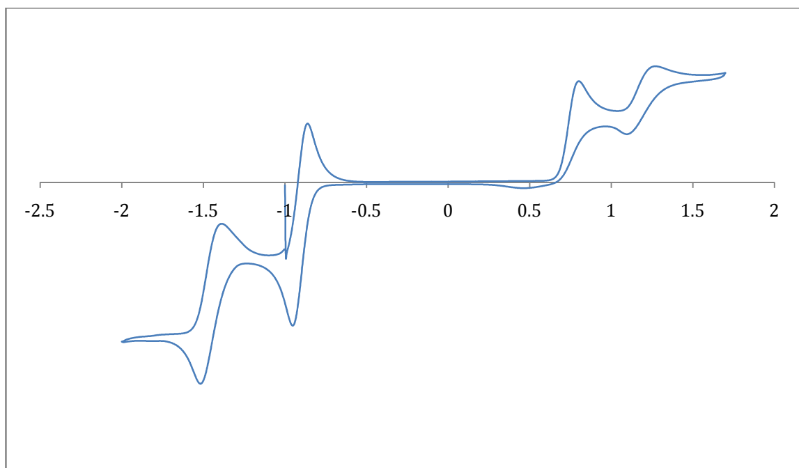
Figure 2 - Cyclic voltammetry scan for (4) - Irreversible oxidation, here at +0.84 V, is typical of the 1-substituted-[4,4'-bipyridin]-1-ium halides, the value varying with the structure of the substituent. The reversible redox processes noted are also typical of these materials, varying in potential with structure of the substituent
