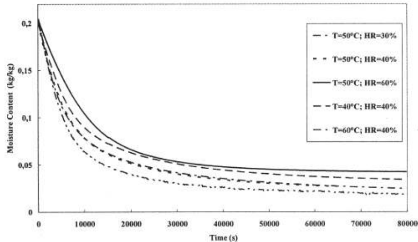
Fig. 6. Drying of clay at different conditions
