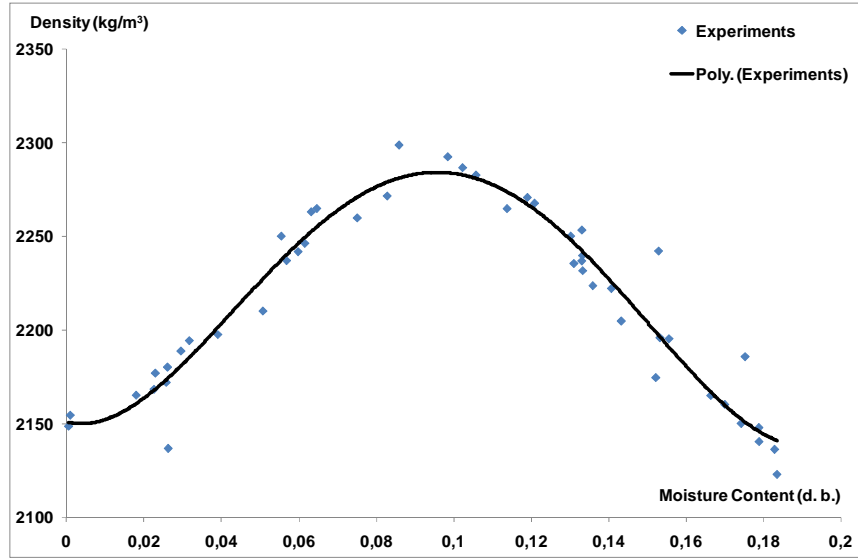
Fig. 7. Clay density versus moisture content.
