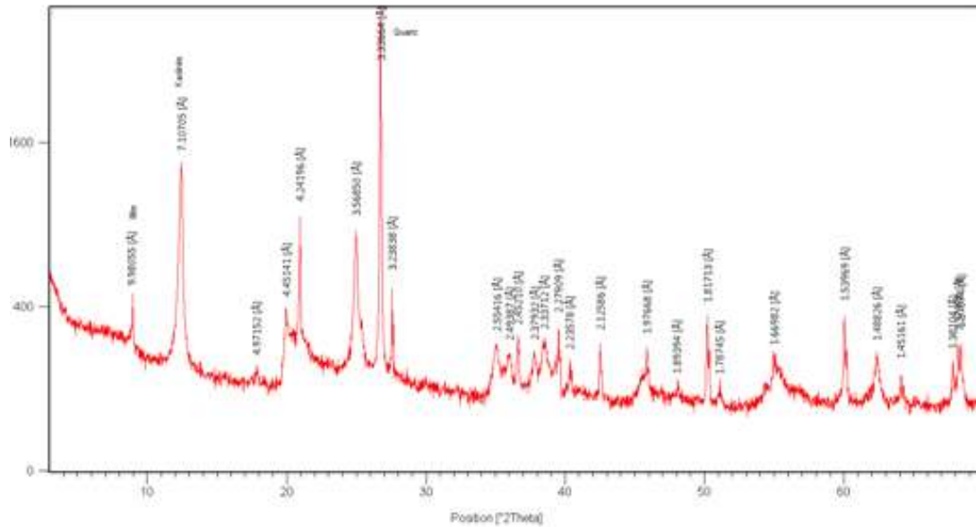
Fig. 5. X-ray diffraction pattern for clay
