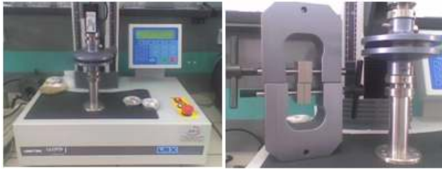
158 Fig.3. Traction compression machine (LRX Plus) with console (Ref. No. 01/2962).
