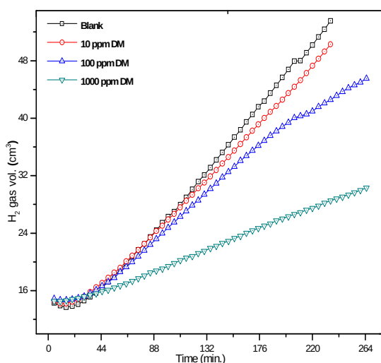
Figure 5 Variation of the volume of H 2 gas evolved with time for FE164531 carbon steel corrosion in 2 M HCl solutions with and without different concentrations of D. mespiliformis leaves extract
