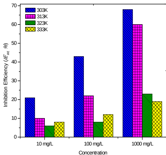
Fig. 7 Inhibition efficiency as a function of D. mespiliformis concentration for FE164531 carbon steel in 2 M HCl solutions at varying temperature obtained from weight loss results
