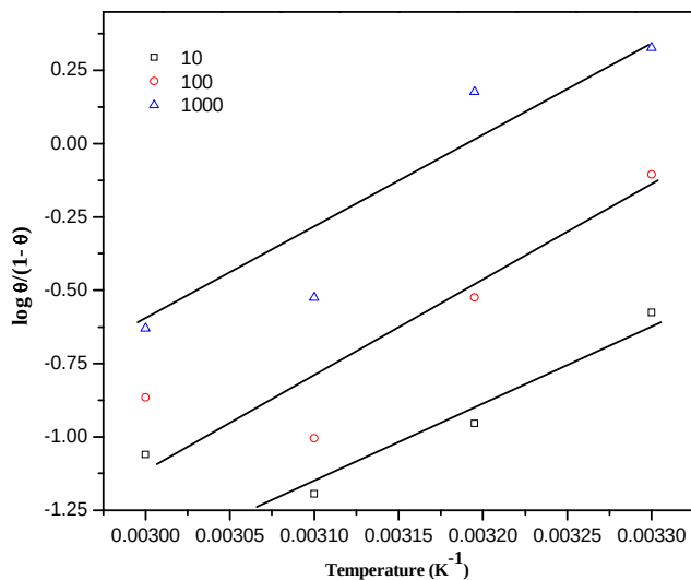
Fig. 8 Heat of adsorption plots as a function of temperature
