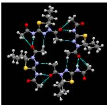
Figure 2: Packing of the molecules of 2j along b-axis
