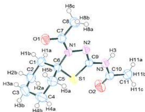
Figure 1: ORTEP diagram of 2j.
