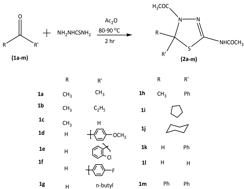
Scheme 1. Synthesis of 1, 3, 4-thiadiazole derivatives via three components approach.
