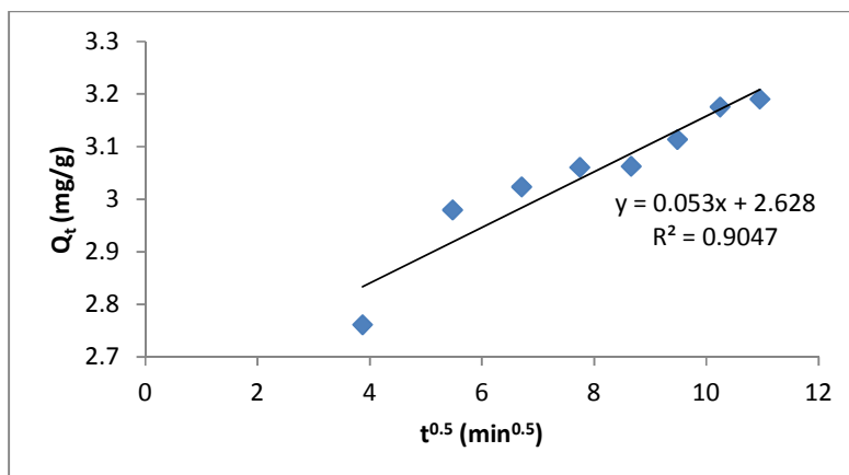
Figure 7: Intra Particle Diffusion Model for the removal of Cyanide ions by SBSH Carbon Black (Process Conditions: pH: 10; Temp. 30°C; Adsorbent Dosage: 3.0g/100ml; ICC: 100mg/L; rpm: 120)
