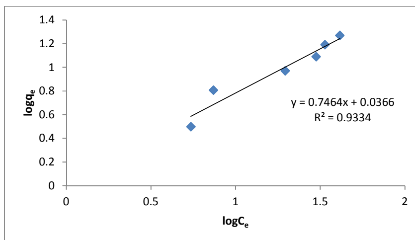
Figure 2: Halsey – Taylor (Freundlich) Adsorption Isotherm for the removal of Cyanide ions (Process Conditions: pH: 10; Temp. 30°C; Adsorbent Dosage: 3.0g/100ml; Contact Time: 120 mins; rpm: 120)
