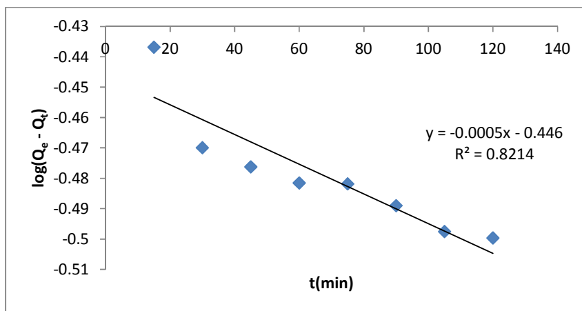
Figure 5: Pseudo-First Order Model for the removal of Cyanide ions by SBSH Carbon Black (Process Conditions: pH: 10; Temp. 30°C; Adsorbent Dosage: 3.0g/100ml; ICC: 100mg/L; rpm: 120)
