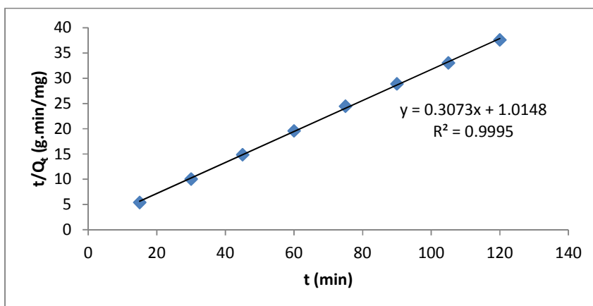
Figure 6: Pseudo-Second Order Model for the removal of Cyanide ions by SBSH Carbon Black (Process Conditions: pH: 10; Temp. 30°C; Adsorbent Dosage: 3.0g/100ml; ICC: 100mg/L; rpm: 120)
