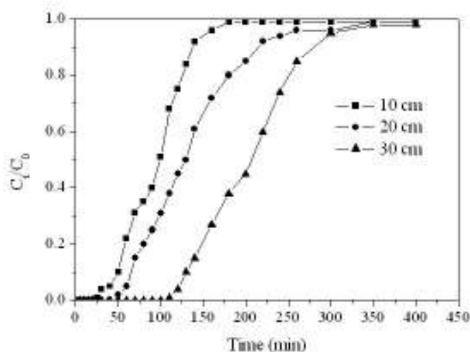
233 Fig. 7 Breakthrough curves for adsorption of Fe(III) onto oxidized MWCNTs at different bed depths.
