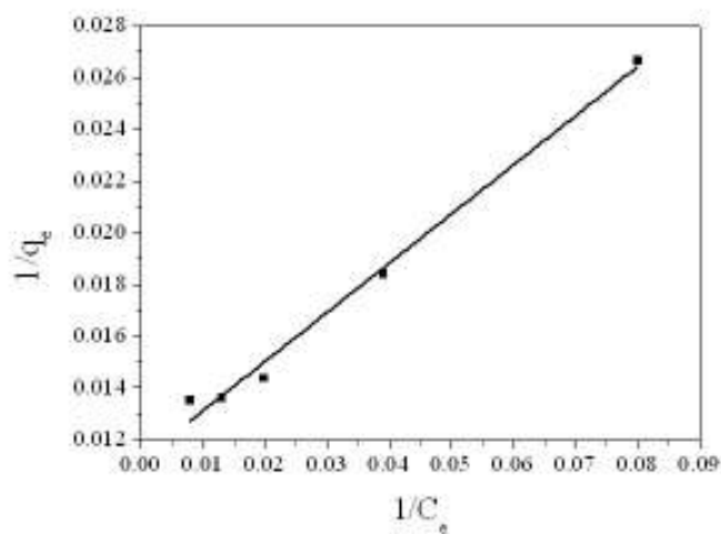
Fig. 5 Langmuir isotherm of Fe(III) adsorption to MWCNTs
