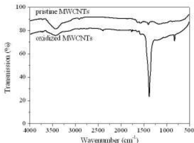
Fig. 1 FTIR spectra of pristine and oxidized MWCNTs
