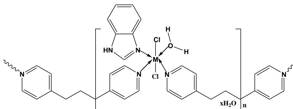
Figure 2. Suggested structure of \{[M(DPP)(BIMZ)(H_2O)Cl_2].xH_2O\}_n M = Mn(II), Co(II), Cu(II) and Cd(II) x = 0 or 1 .
