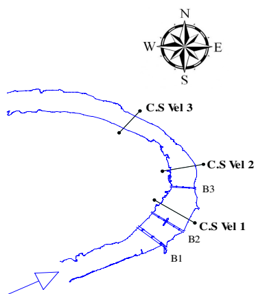
Fig. 4. Location of the Calibration Cross Sections
