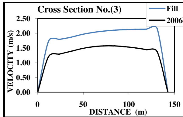
Fig. 14. Cross Sections Velocity Profile of the Original & Alternative (1) at Future Flow
