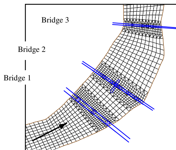
Fig. 3. Mesh Generation
