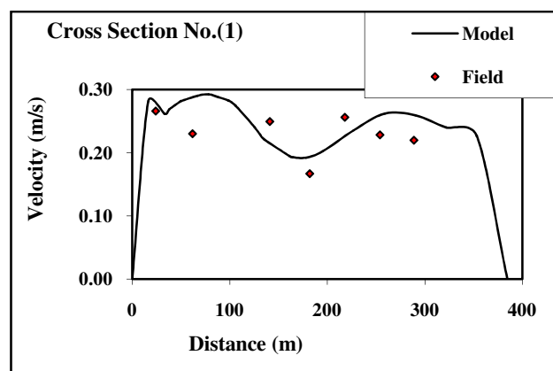
Fig. 5. Flow Velocity Calibration at Cross Section (1)
