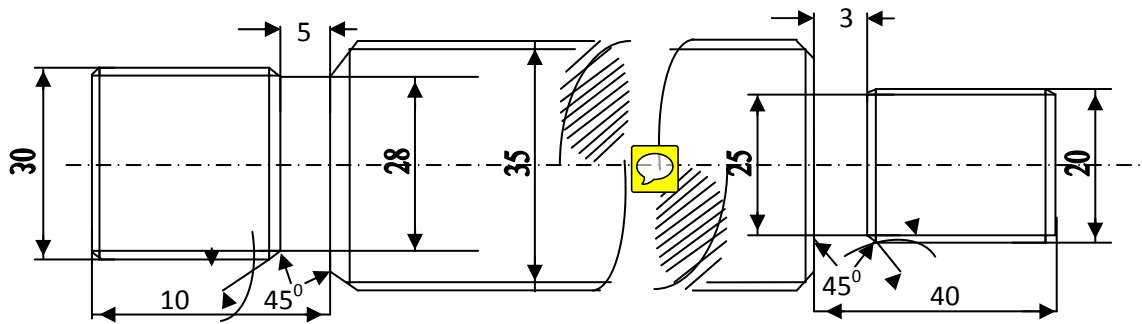
Figure 1: Component to be Manufacture and its Geometry
