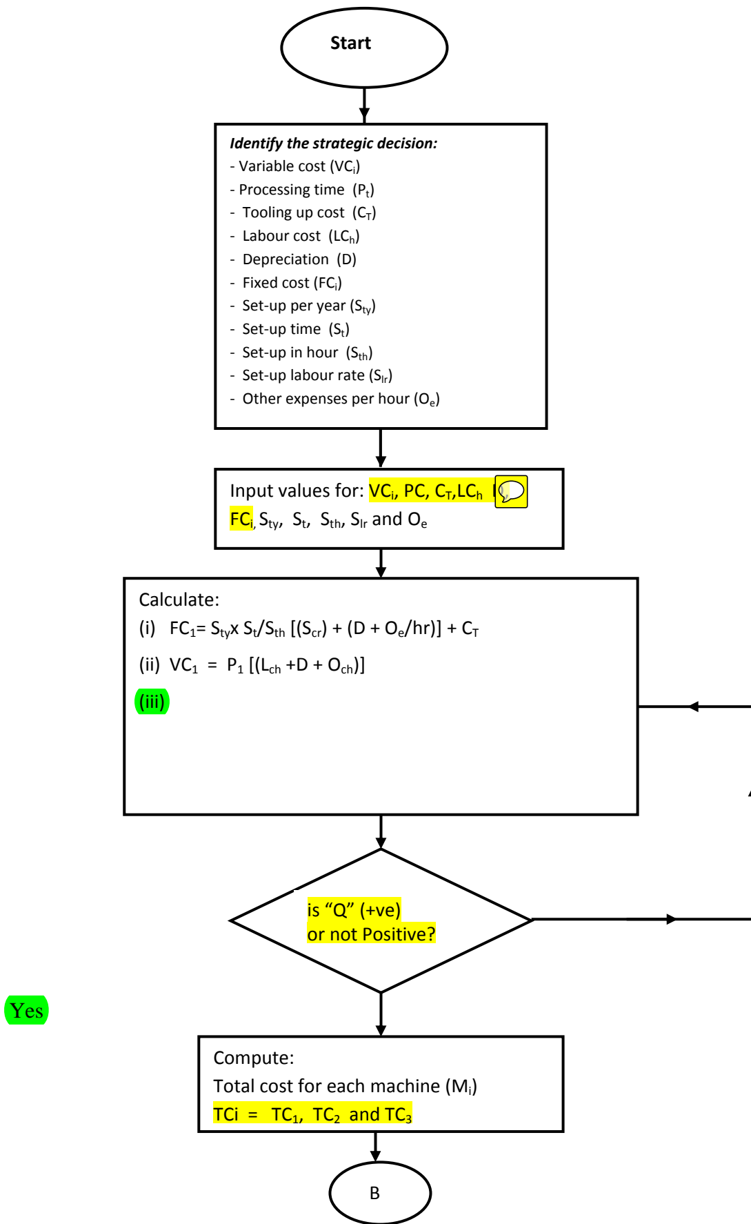
Fig. 2 Software Logic
