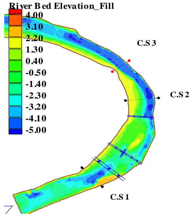
Fig. 11. River Bed Elevation in the Case of Alternative (1)
