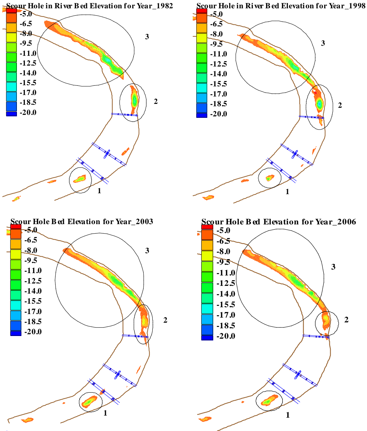
Fig.9. Scour Holes Location in the Study Area at Years 1982, 1998, 2003 & 2006
