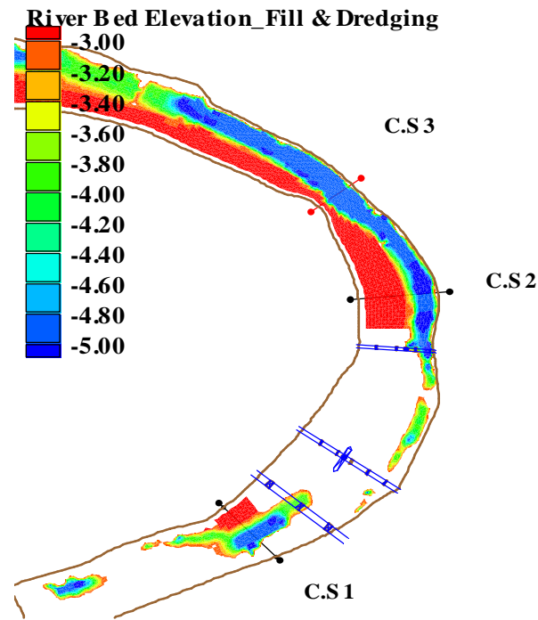
Fig.15. River Bed Elevation in the Case of Alternative (2)
