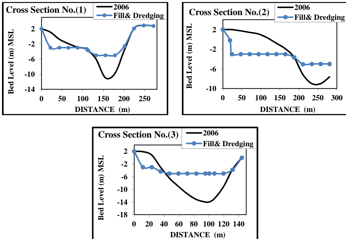
Fig.16. Bed Profiles at Different Cross Sections for the Basic Case and Alternative (2)
