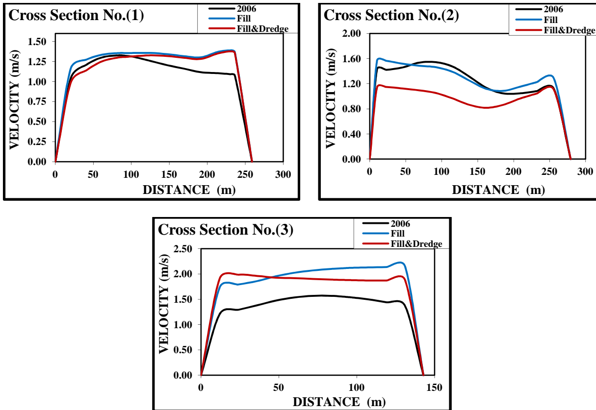
Fig.18. Velocity Profiles for the Basic, Alternatives (1) and (2) at Emergency Flow
