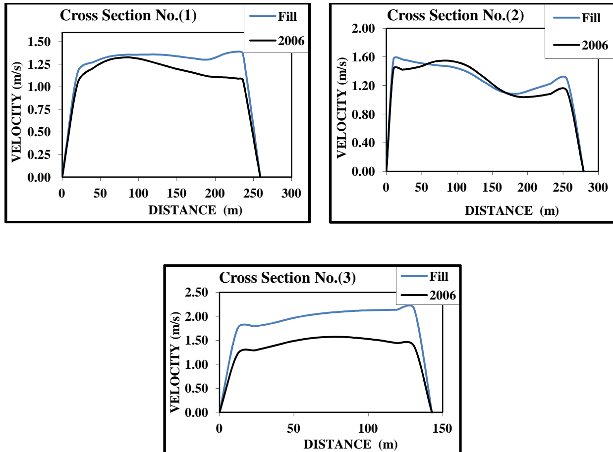
Fig.14. Velocity Profiles for the Basic & Alternative (1) at Future Flow Conditions
