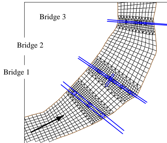
Fig.3. Mesh Generation
