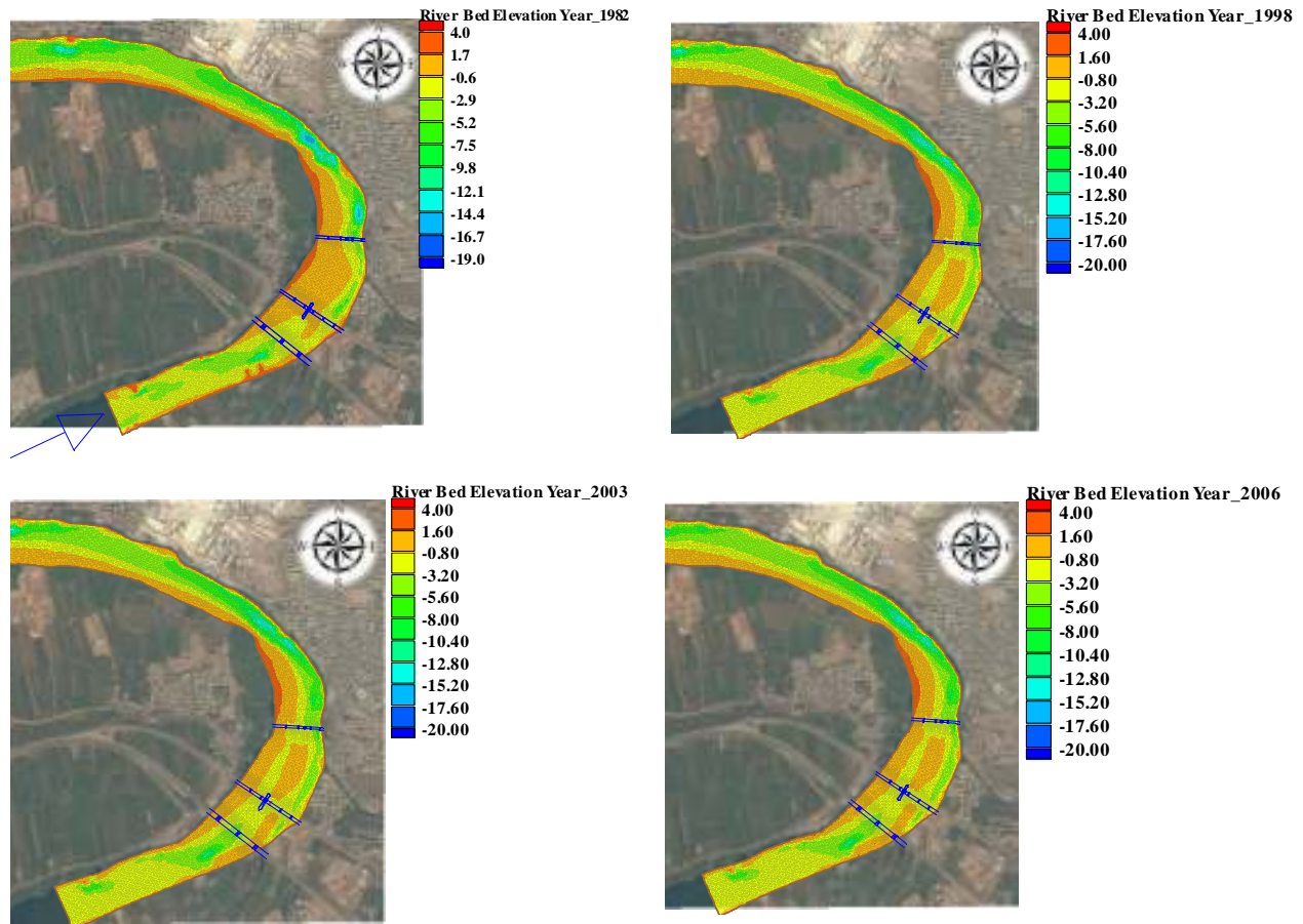
Fig.8. River Bed Elevation at Years 1982, 1998, 2003 and 2006
