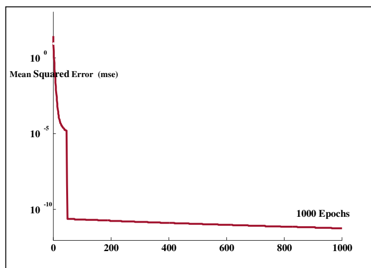
Figure 4. The iteration-dependent error graph of an ANN prepared for training.
