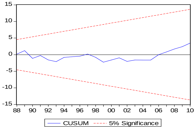
Fig. 3a. CUSUM plot of residuals
