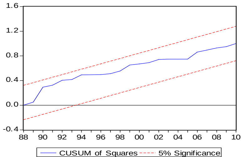
Fig. 3b: CUMUQ plot of residuals.
