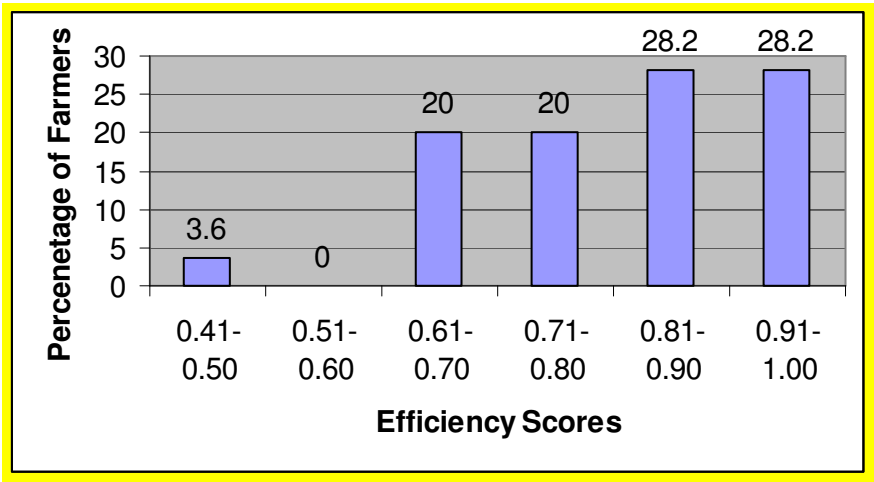
Figure 1: Frequency distribution of technical efficiency scores
