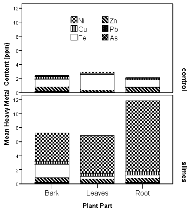
Fig 5. Heavy metal contents in the plant parts.
