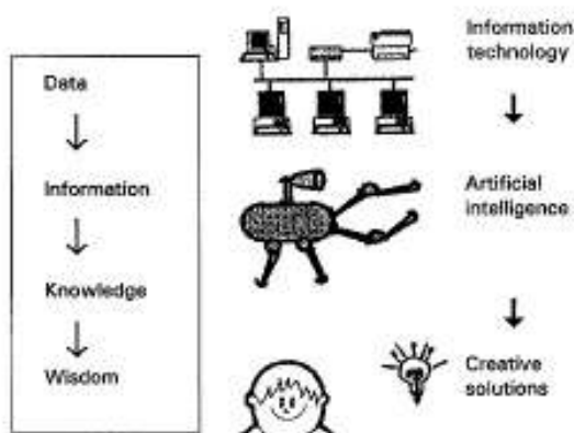
229 230 Fig. 3: Information level (Shibusawa 1999, 2000)
