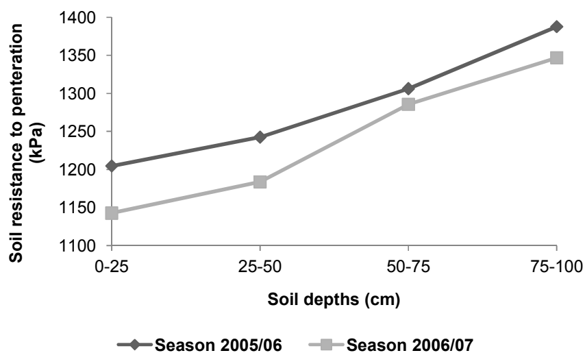
Fig. 3. Soil resistance to penetration (kPa) at different soil depths (cm) of the experimental site before tillage for both seasons
