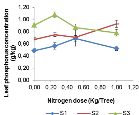
Figure 4. Leaf phosphorus concentration as a function of nitrogen applications in the three sites.
