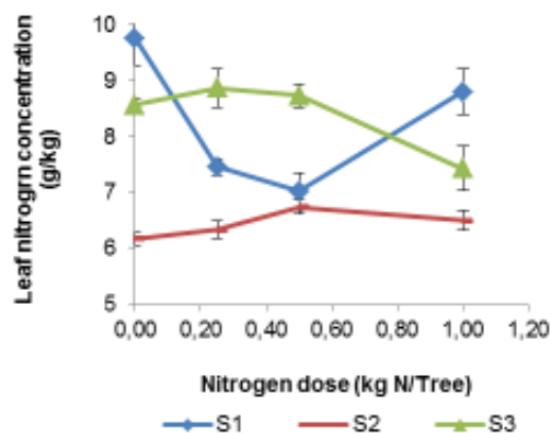
Figure 3. Leaf nitrogen concentration as a function of N rate in the three sites.
