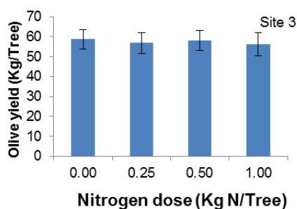
Figure 2. Olive response to nitrogen fertilizer in the three sites
