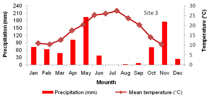
Figure 1. Monthly precipitation and temperature recorded during the 2011 campaign in the three sites.
