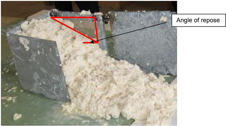
Figure 2: Mash flowing from the box
