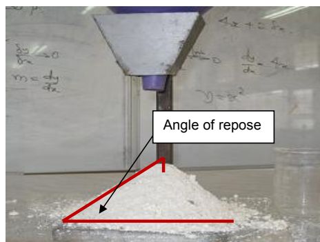
Figure 3: Measuring the angle of repose for pulverized mash.
