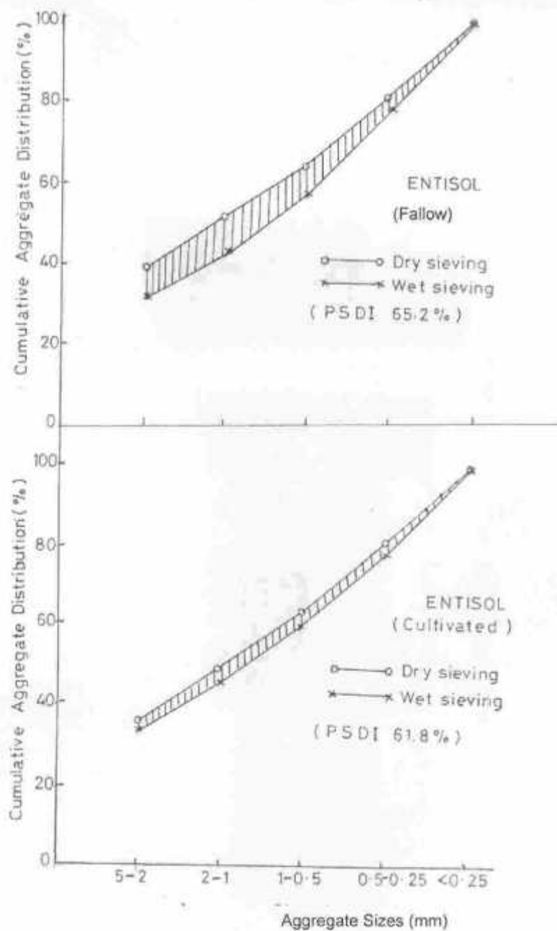
FIG 1: Distribution of aggregate obtained from dry and wet sieving procedures in an Entisol (Nsukka Hill Site) under different lands uses. (PSDI=Potential structure deformation index)
