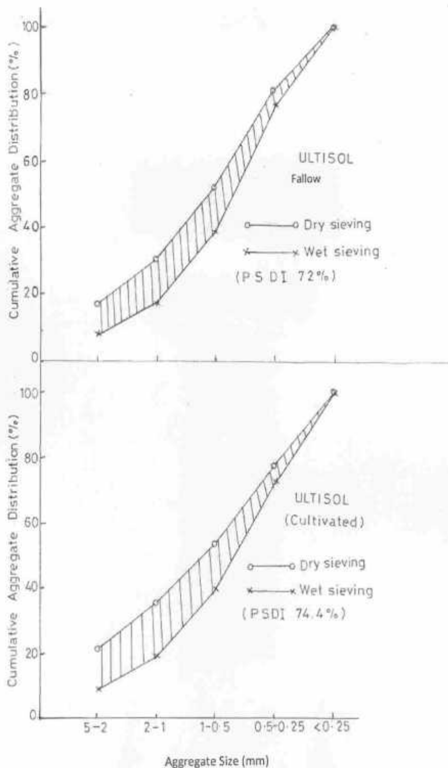
FIG 2: Distribution of aggregate obtained from dry and wet sieving procedures in an Ultisol (Nsukka Poultry site) under different land uses. (PSDI=Potential structural deformation index)
