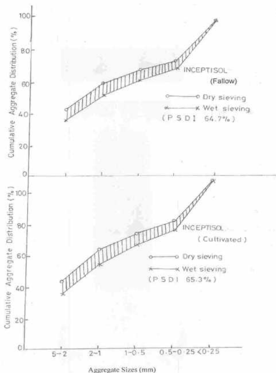
FIG 4: Distribution of aggregates obtained from dry and wet sieving procedures in an inceptisol (Ikem site) under different uses. (P SDI= Potential structural deformation index)
