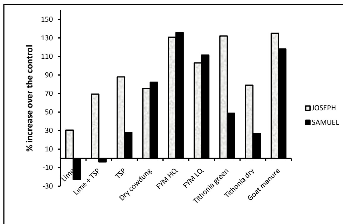
163 Figure 1. % Increase in drymatter yield over the control
