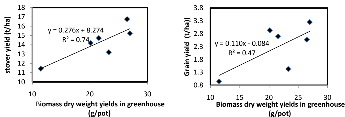
Figure 3. Relationship between biomass dry weight yield (Joseph's soil) in greenhouse with stover and grain yields in the field.
