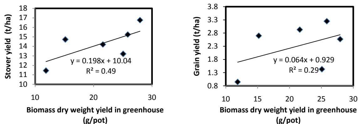
Figure 4. Relationship between biomass dry weight yield (Samuel's soil) in greenhouse with stover and grain yields in the field.
