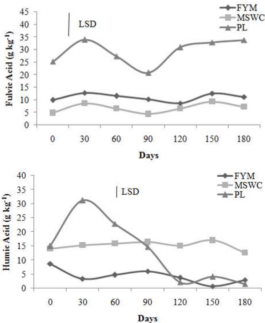
Figure 3: Dynamics of humic carbon fractions (Humic acid and Fulvic acid) in different organic matter sources during 180 days of incubation
