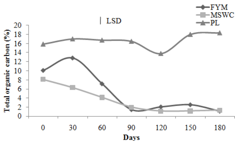
Figure 1: Dynamics of TOC in different organic matter sources during 180 days of incubation.
