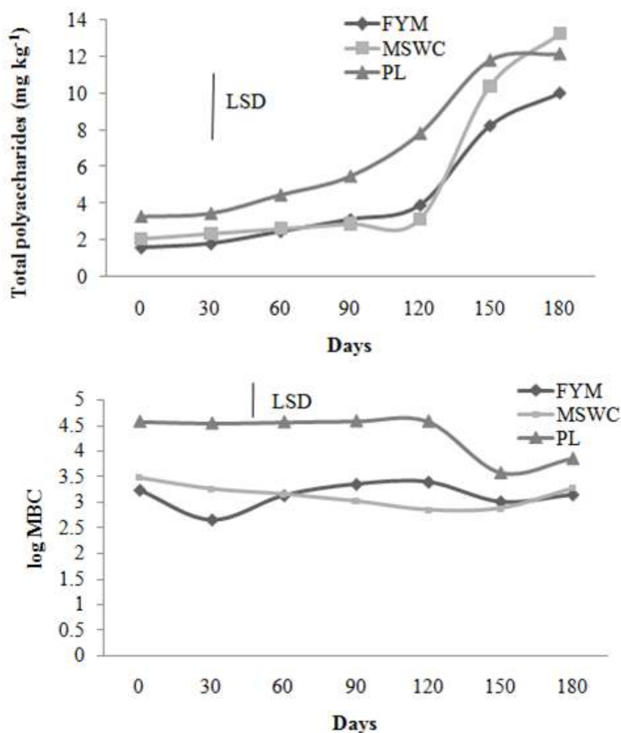
Figure 2: Dynamics of non humic carbon fractions (TPC and MBC) in different organic matter sources during 180 days of incubation
