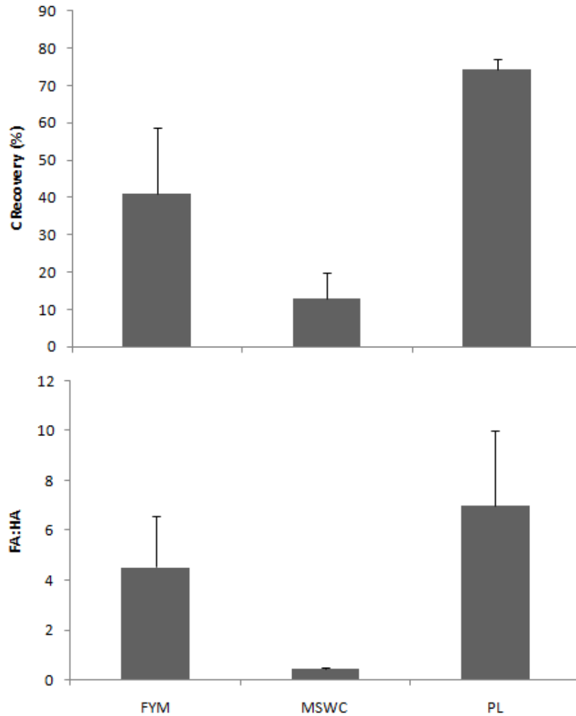
Figure 4: Carbon recovery and FA:HA ratio in different organic matter sources averaged over 180 days.
