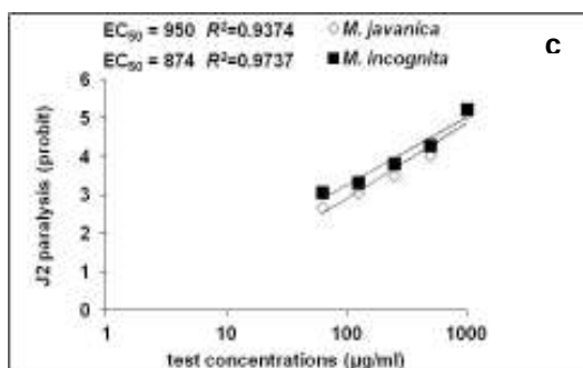
Figure 2. Regression curves of M. incognita (a) and M. javanica (b) paralysis following J2 immersion in solutions of extract C-4, for 24 h and 48 h and J2 immersion for 48 h in solution of extract C-4 after exhaustive evaporation of solvents (c). Each point represents the average % number of paralyzed J2 of five replications per treatment (two experiments replications) after elimination of natural paralysis/death observed in the control.
