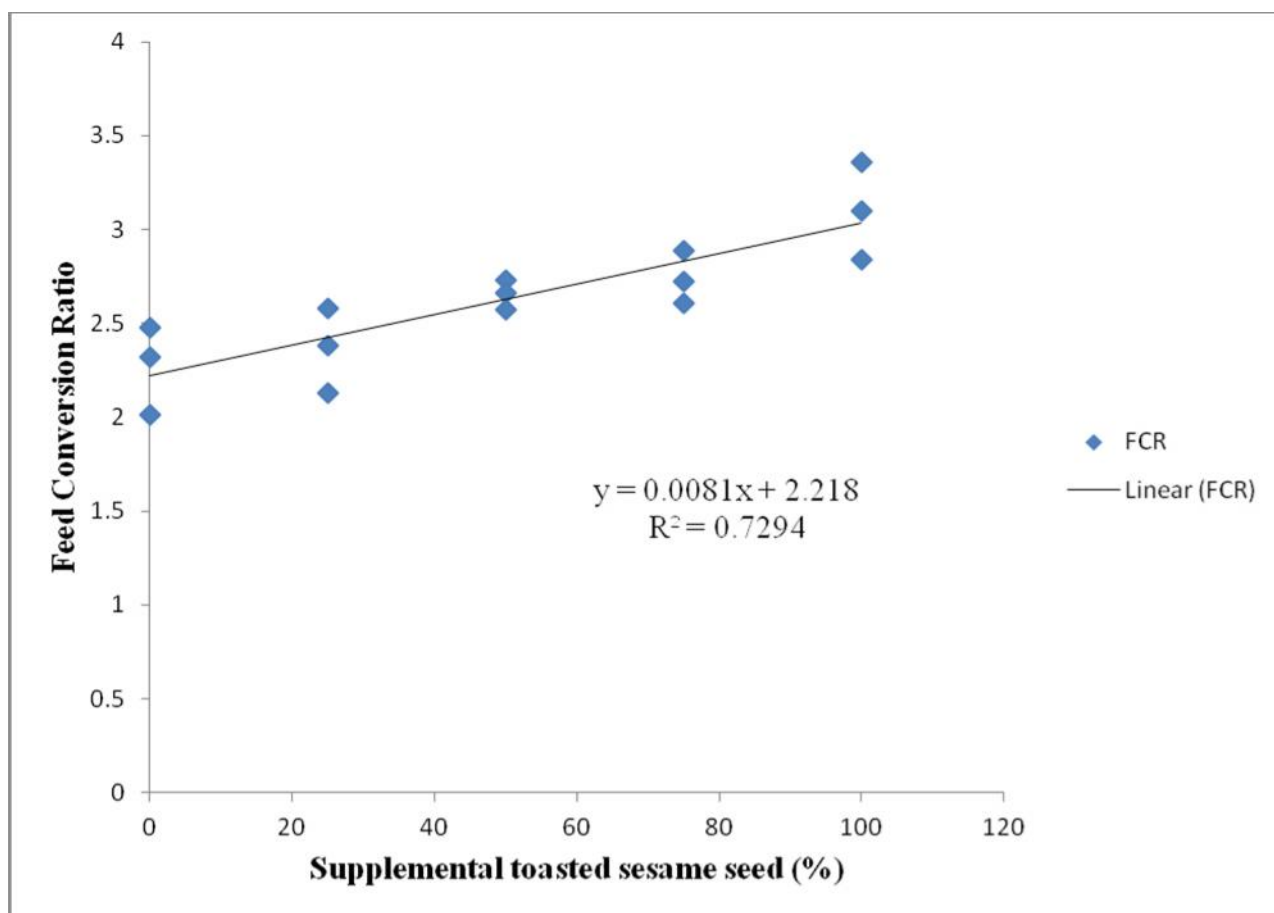
Figure 2: Relationship between supplemental graded toasted sesame seed and feed conversion ratio of broilers fed experimental diets
