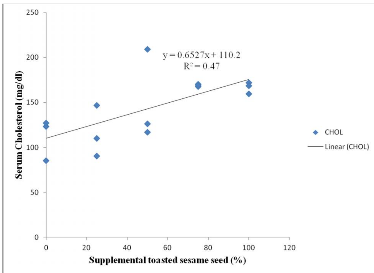
Figure 5: Relationship between supplemental graded toasted sesame seed and serum cholesterol of broilers fed experimental toasted sesame seed diets
