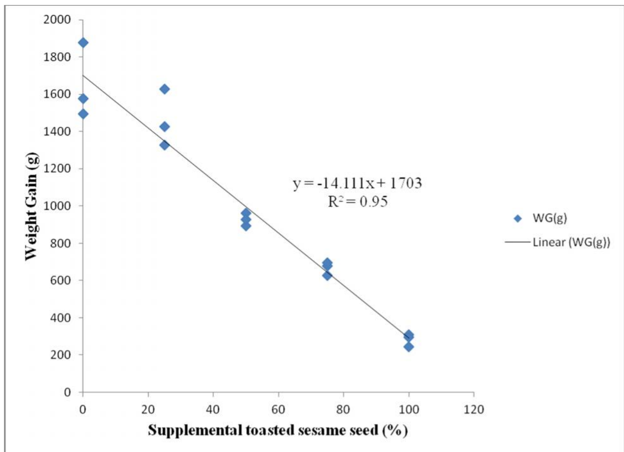
Figure 1: Relationship between supplemental graded toasted sesame seed and weight gain of broilers fed experimental diets
