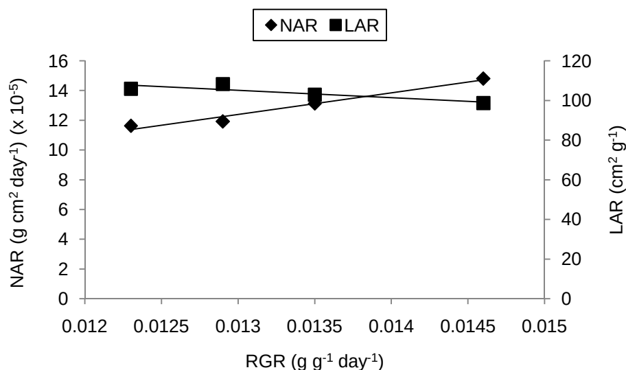
Fig. 2. Changes in the net assimilation rate (NAR) and the leaf area ratio (LAR) related to the relative growth rate (RGR). The straight-line regressions were: \text{NAR} \times 10^{-5} = 1.45 \text{ RGR} - 6.46 ( r^2 = 0.972 ) and \text{LAR} = -3.71 \text{ RGR} + 153.32 ( r^2 = 0.773 ).
