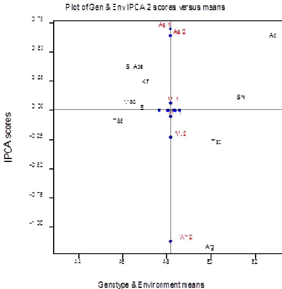
Fig. 2. AMMI Biplot for Oil Content (%)
