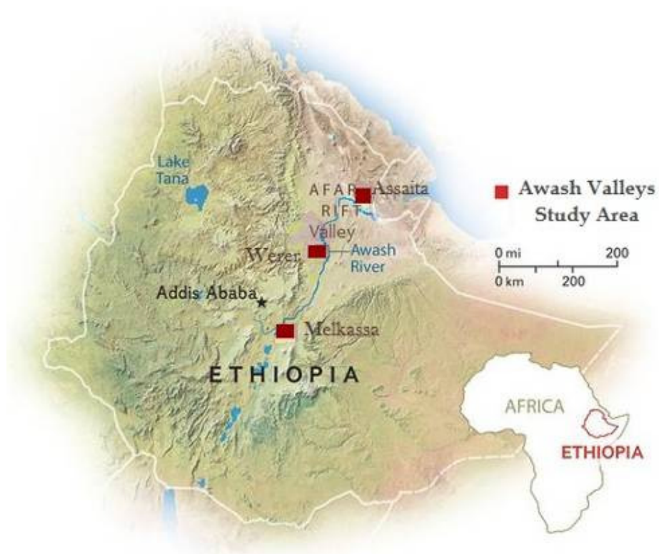
Fig. 1 Maps locating the study areas: Upper, Middle and Lower Awash valleys in Ethiopia.
