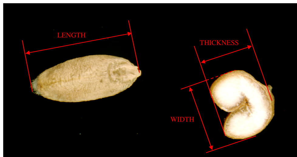
Fig. 1. Images of wheat kernel surface and cross-section with a indication of the dimensions measured by the digital image analysis
