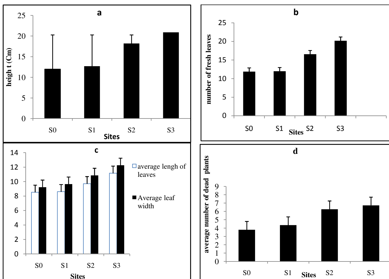
Fig. 2. Evolution of growth parameters of Lactuca sativa L. (a: height of plant; b: number of fresh leaves; average length and average width of leaves, d: average number of dead plants).
