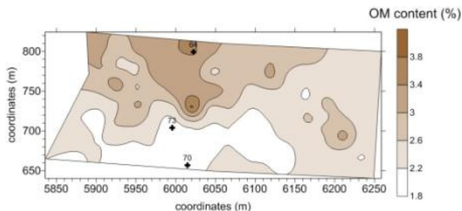
Fig. 1. Agricultural field with different soil sampling points (64, 70, 73) varying in soil organic matter content (OM)
