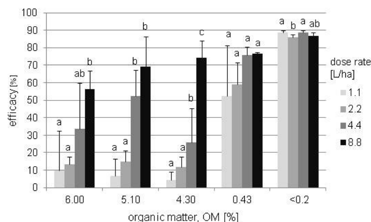
Fig. 2. Herbicidal effects of different concentrations of pendimethalin against Stellaria media in soils with varying organic matter content. Columns with different letters are significantly different, according to one-way ANOVA
