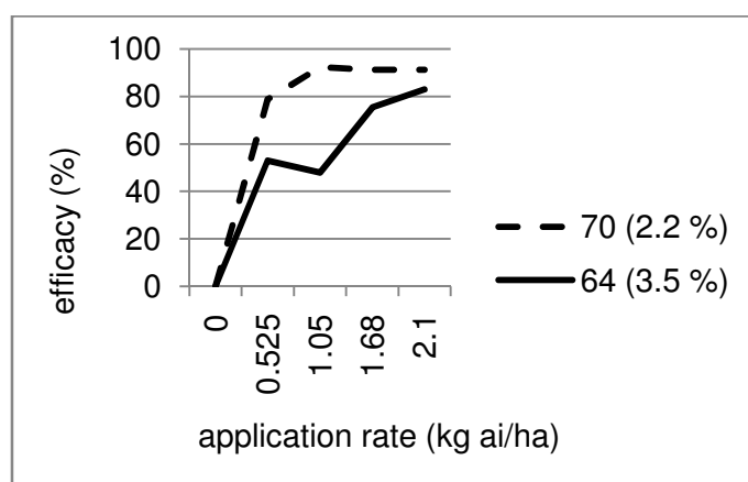
Fig. 3. Efficacy of chlorotoluron against Alopecurus myosuroides
