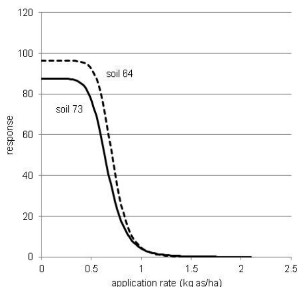
Fig. 3. Efficacy of chlorotoluron against Alopecurus myosuroides
