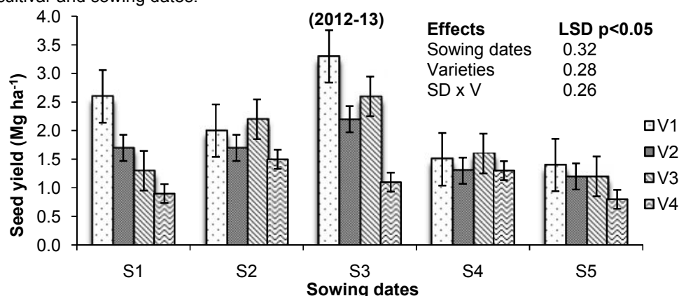
Figure. 3: Sowing dates and varieties effects seed yield (Mg ha -1 ) of chickpea (data over 2012-13). (S 1 = 15 th October 2012, S 2 = 30 th October 2012, S 3 =15 th November 2012, S 4 = 30 th November 2012 and S 5 =15 th December 2012. V 1 = DG-92, V 2 = Chhola, V 3 = DG-89 and V 4 = Sanyasi).
