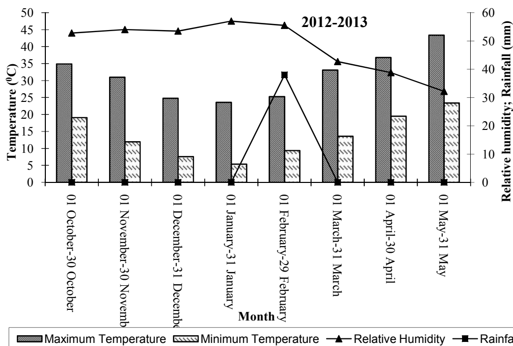
Figure 1: Meteorological data recorded at Rice Research Institute, Dokri, during Rabi season, 2012-13.
