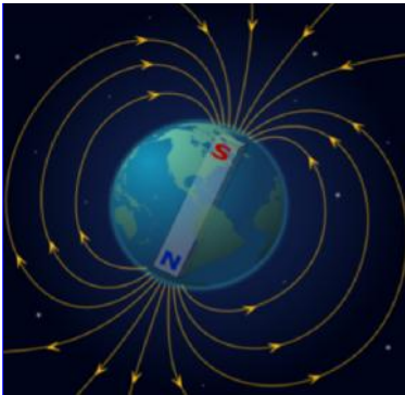
Fig 5. Earth's magnetic field and magnetic field around permanent magnets.
