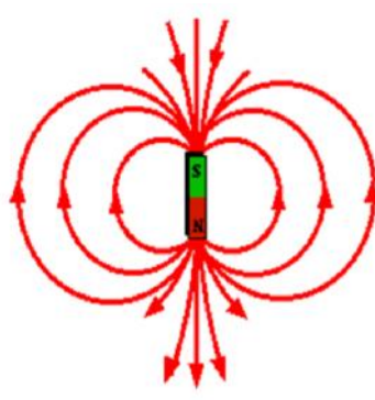
Fig 5. Earth's magnetic field and magnetic field around permanent magnets.
