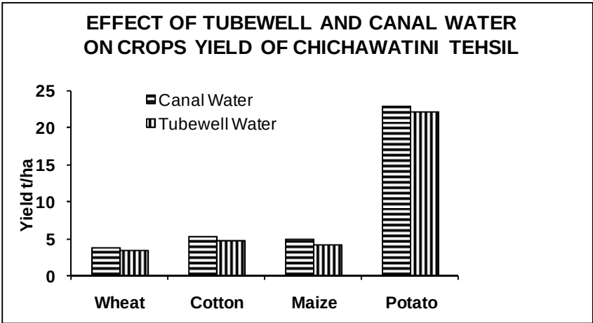
172 Fig.4. Effect of water quality on the yields of crops at farmer's fields in Chichawatni tehsil of District Sahiwal. EC of TW 173 ranged from 1.00 to 2.82 dS m -1 ; SD for wheat, cotton, maize and potato yields in canal irrigated fields were \pm 0.61 , 174 \pm 0.77 , \pm 0.19 and \pm 1.85 ; and in tubewell irrigated fields were \pm 0.57 , \pm 0.72 , \pm 0.13 and \pm 1.20 , respectively.
