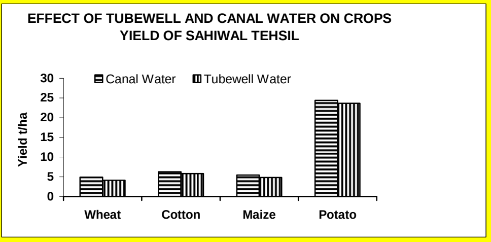
177 Fig.5. Effect of water quality on the yields of crops farmer's fields in Sahiwal tehsil of District Sahiwal. EC of TW ranged 178 from 1.12 to 3.62 dS m -1 ; SD for wheat, cotton, maize, potato yields in canal irrigated fields were \pm 0.91 , \pm 0.73 , 179 \pm 0.65 and \pm 1.80 ; and in tubewell irrigated fields were \pm 0.80 , \pm 0.63 , \pm 0.12 and \pm 1.79 , respectively.
