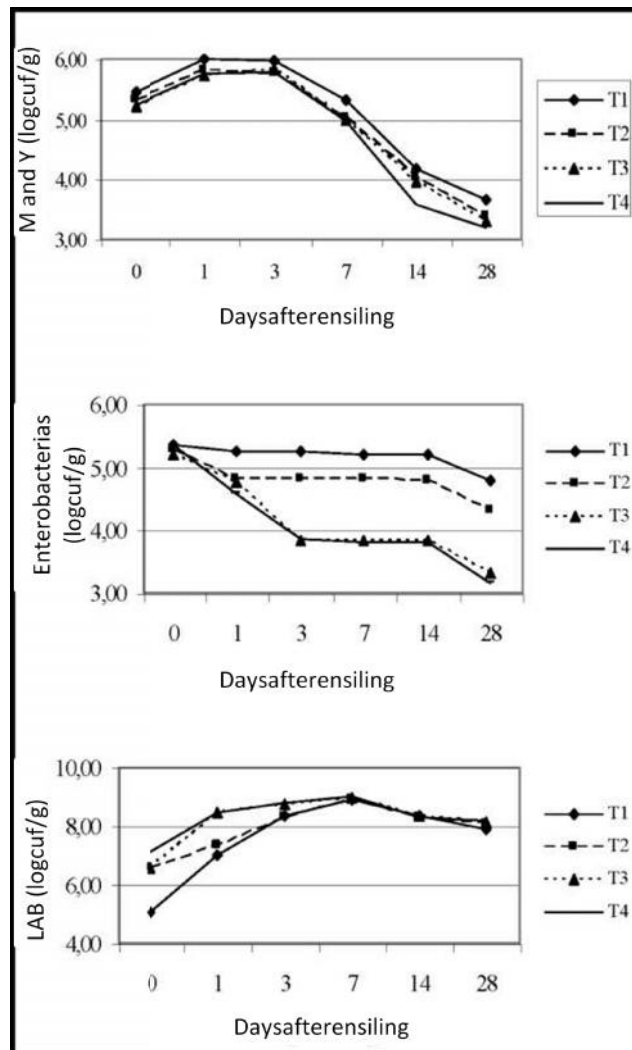
Figure 1. Populations of molds and yeasts (M and Y), enterobacteria and lactic acid bacteria (LB), in mombasa grass silage without inoculant (T1), inoculated with 10^4 CFU/g forage (T2), inoculated with 10^5 CFU/g forage (T3) and inoculated with 10^6 CFU/g forage of Lactobacillus plantarum of epiphytic microbiota.
