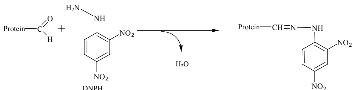
Fig. 2. Derivatisation of carbonyl group with DNPH
