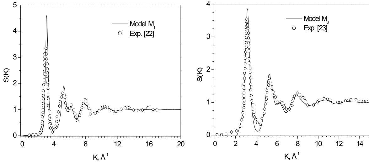
Fig.2. The structure factor Fe (left) and \text{Fe}_{80}\text{B}_{20} (right) amorphous models
