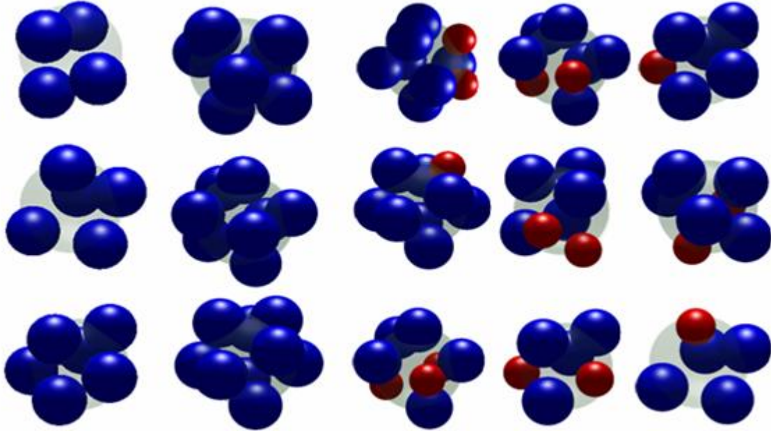
Fig.1. The snapshot of typical simplexes detected in the Fe-based alloys. Blue and red spheres indicate iron and boron atoms, respectively.
