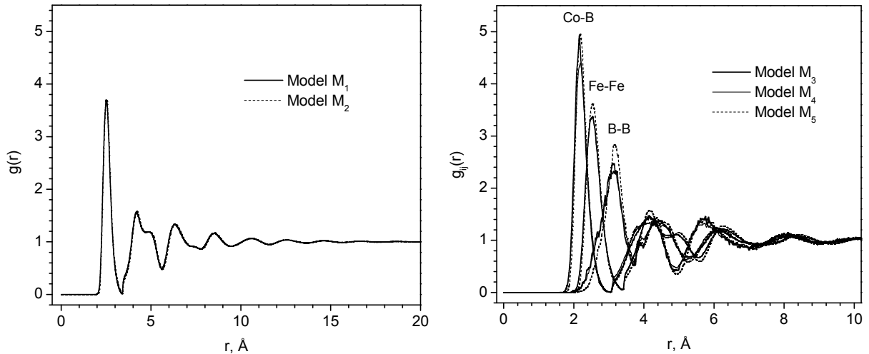
Fig.3. The partial radial distribution functions Fe (left) and \text{Fe}_{80}\text{B}_{20} (right) models
