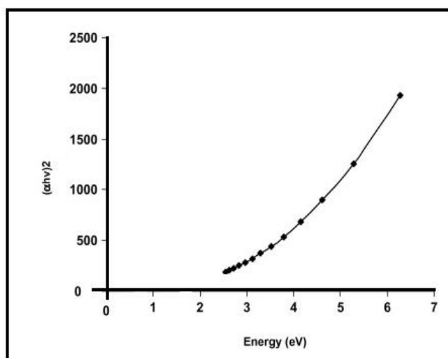
96 97 Fig.2. Band gap of 4-methoxy benzoin crystal 98 99 100 101
