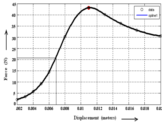
Figure 1 Force versus displacement
