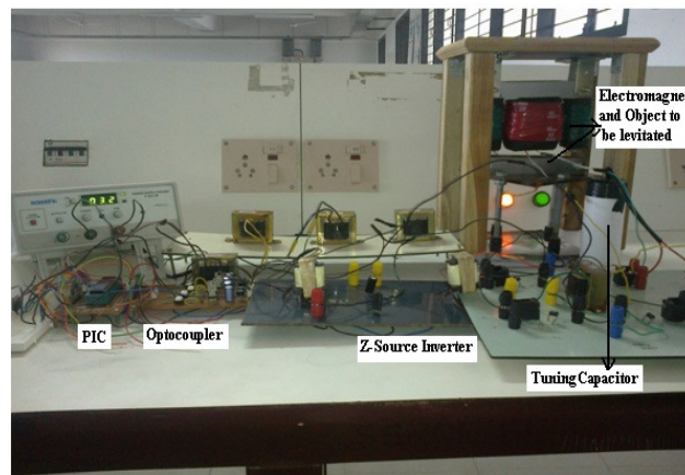
Figure 9 Experimental Set up
