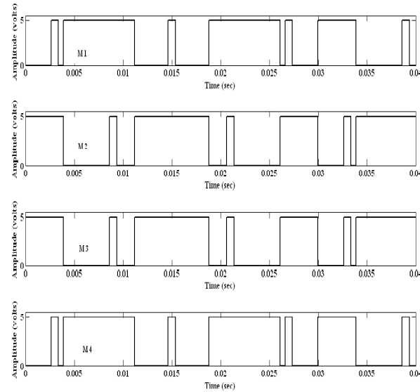
Figure 5 Gating pulses of inverter
