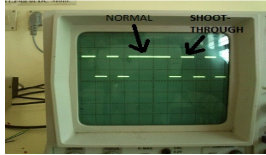
Figure 7 Change in pulse width with change in capacitor voltage
