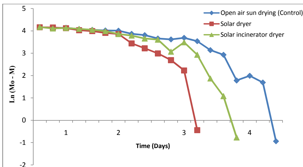
Fig. 4: Drying pattern distribution rates for Pepper drying
