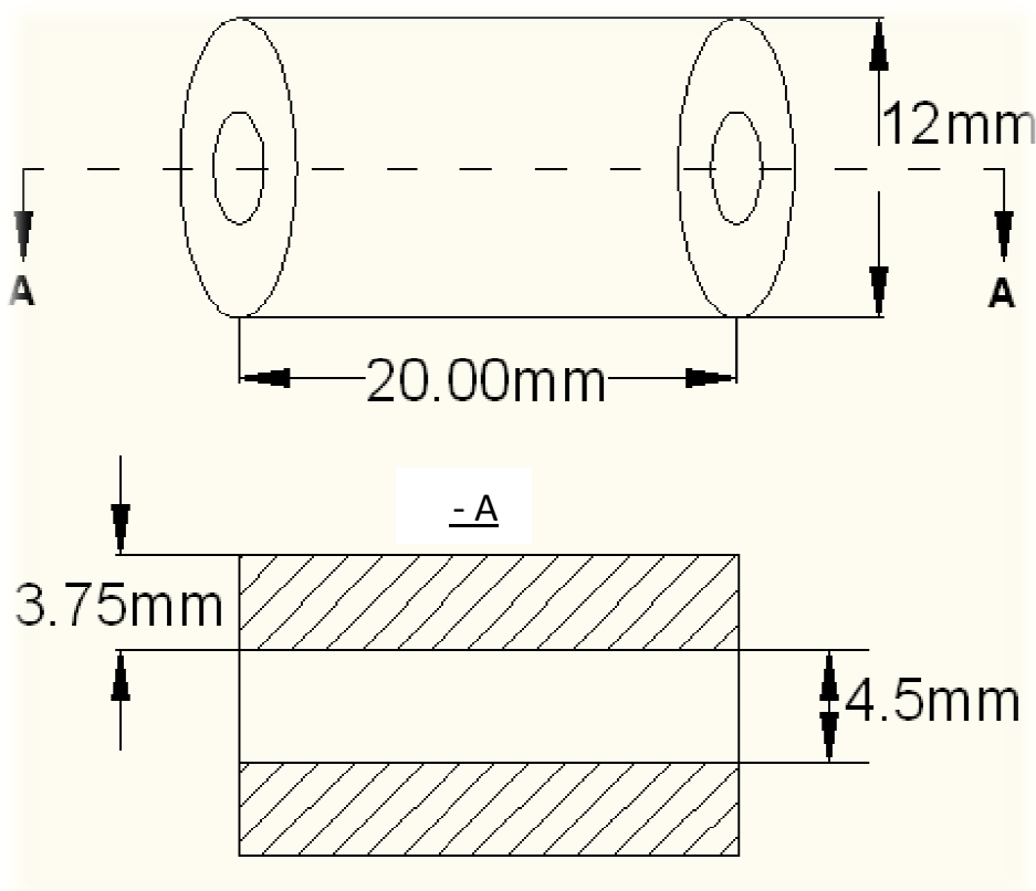
Fig 6 – Nozzle and its cross section
