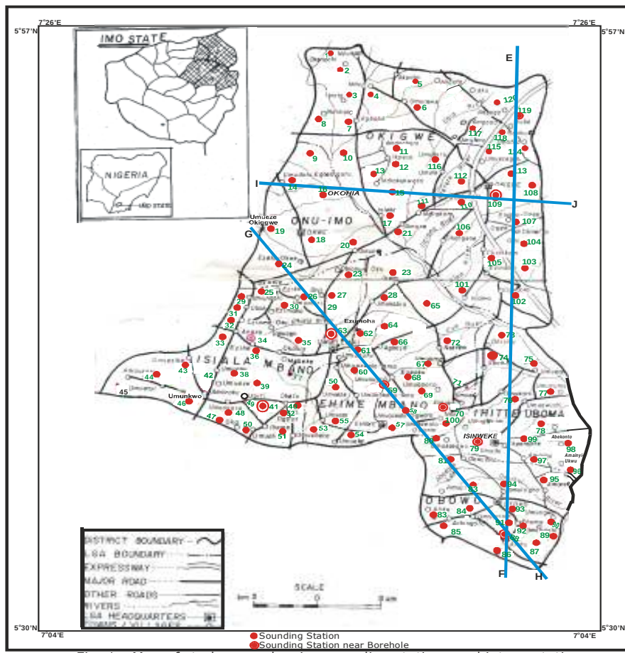
Fig. 5. Interpretative Geoelectric Cross-Section (IGCS) traverse
