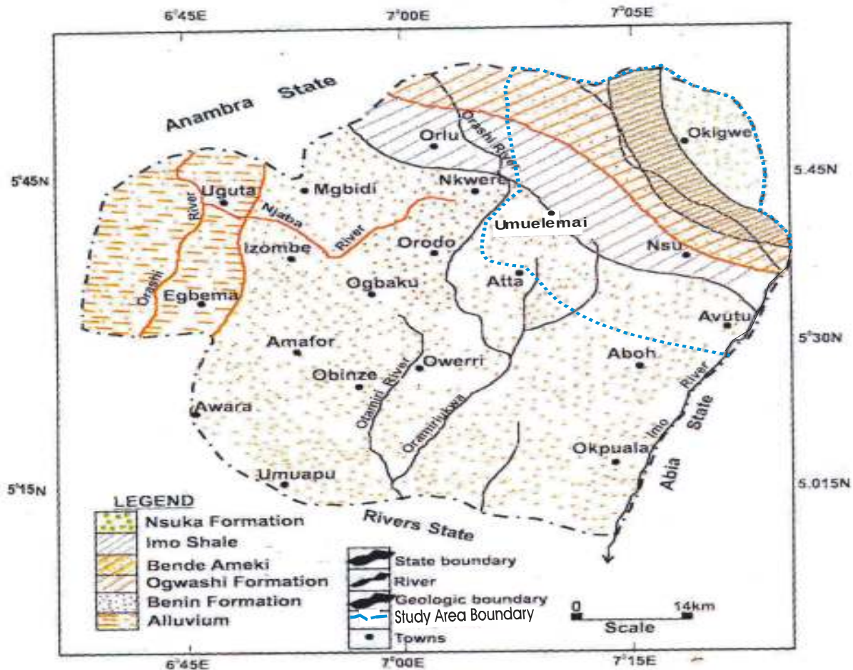
Fig. 2. Geological map of the study area (Adapted from Akolisa and Selemo, 2009)
