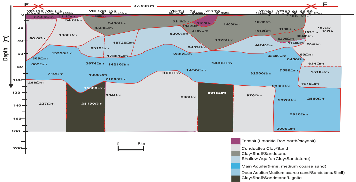
Fig. 6a: Interpretative Geoelectric Cross-Section (IGCS) along profile EF
