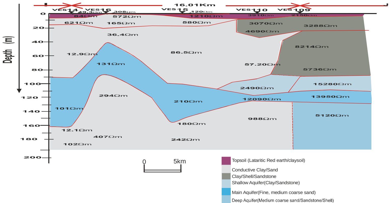
Fig. 6a: Interpretative Geoelectric Cross-Section (IGCS) along profile IJ
