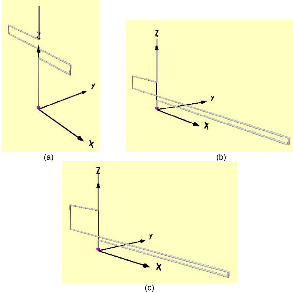
Fig. 5. VSO(a), GA(b), and SAHC(c) Optimized DLM (0.2 m axis length, 299.8 MHz).
