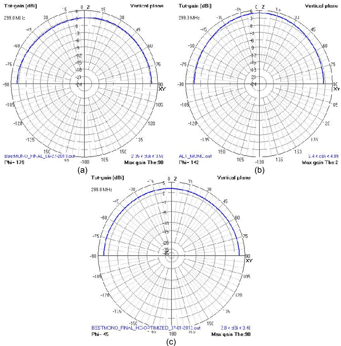
Fig. 7. Optimized DLM Radiation Patterns: VSO(a), GA(b), SAHC(c)
