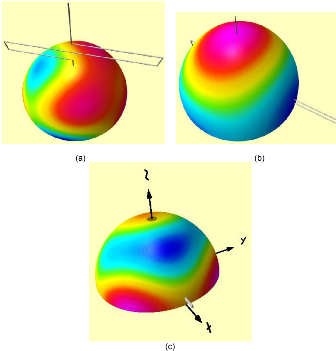
Fig. 8. Optimized DLM 3-D Patterns: VSO(a), GA(b), SAHC(c)
