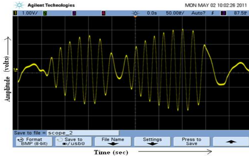
Figure 2 Waveform during vibrations
