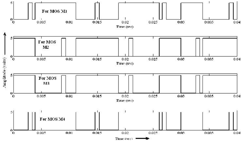
Figure 5 Gating pulses of inverter
