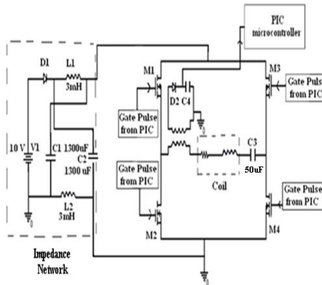
Figure 3 Schematic of the system developed
