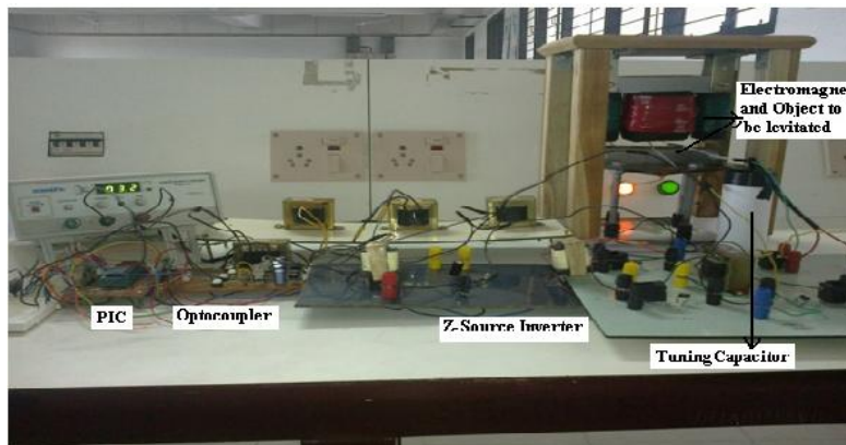
Figure 9 Experimental Set up
