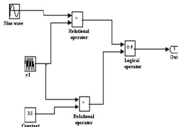
Figure 4 SIMULINK model for generating gating Pattern
