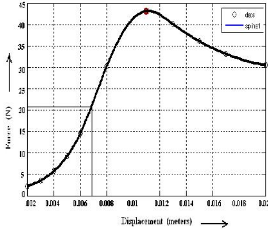
Figure 1 Force versus displacement
