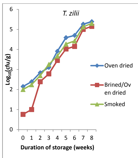
Figs 3: Total viable count ( \text{Log}_{10} cfu/g) of processed Tilapia zillii
