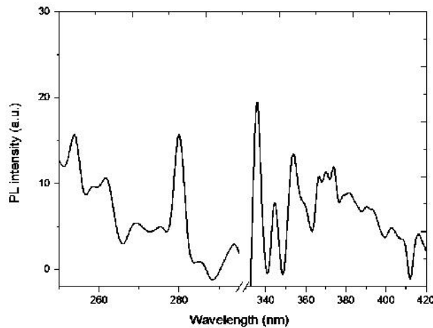
Figure 7(I) Photoluminescence excitation spectra
