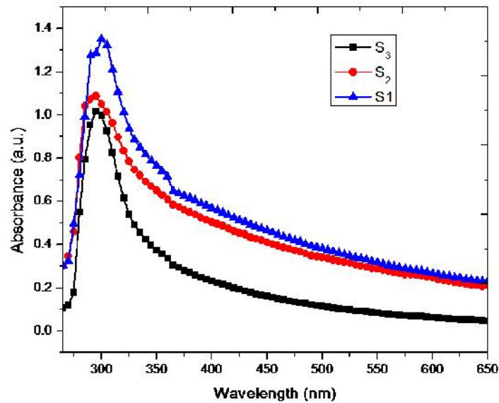
Figure 5 (I) Absorption spectra for S 1 , S 2 and S 3 samples
