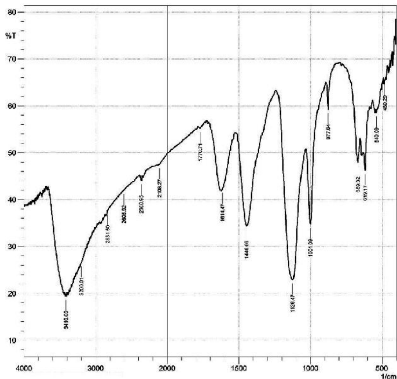
Figure 6(b) FTIR spectrum of S_3 sample
