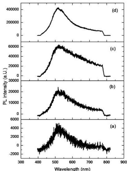
Figure 7(IV) Photoluminescence emission of S 2 sample at (a) 320 nm, (b) 345 nm, (c) 365 nm and (d) 394 nm excitations
