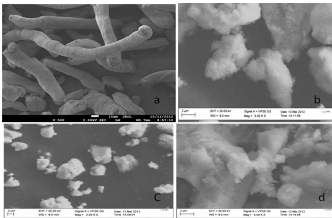
Figure 2 SEM micrographs of (a) CMC, (b) \text{S}_1 , (c) \text{S}_2 and (d) \text{S}_3 samples.
