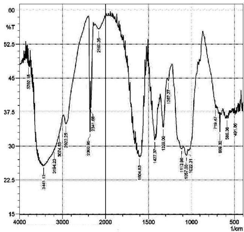
Figure 6(a) FTIR spectrum of the CMC sample
