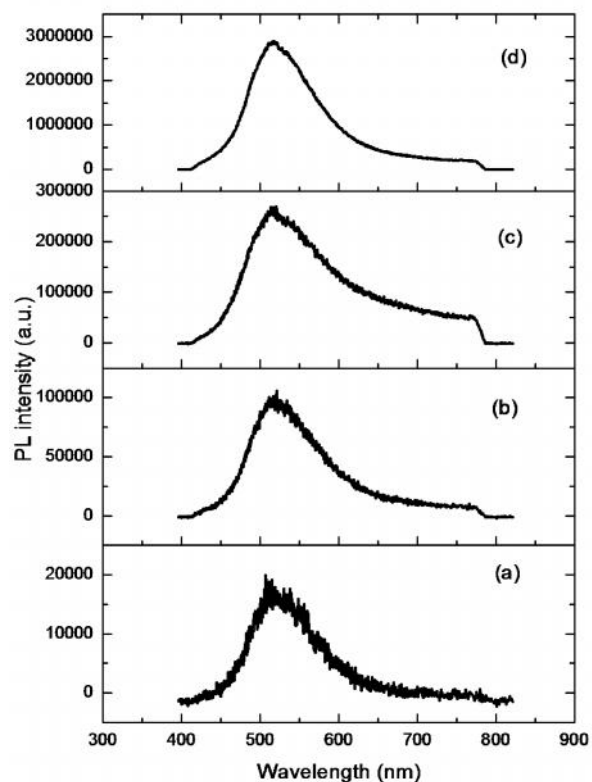
Figure 7(III) Photoluminescence emission of sample S_2 at (a) 320 nm, (b) 345 nm, (c) 365 nm and (d) 394 nm excitations
