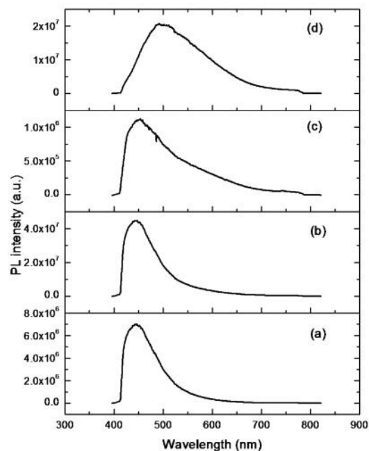
Figure 7(II) Photoluminescence emission of sample S_1 at (a) 320 nm, (b) 345 nm, (c) 365 nm and (d) 394 nm excitations
