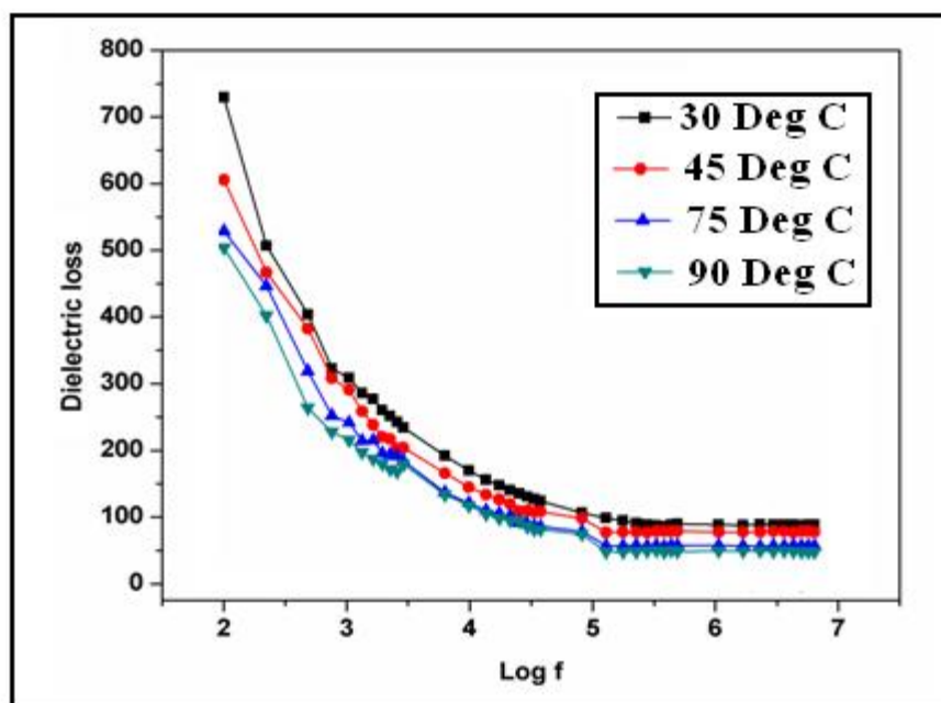
Fig.4 Variation of the dielectric loss with log f
