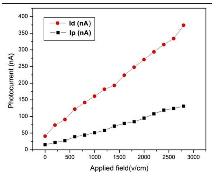
Fig. 5 Dark current and photocurrent as a function of the applied field
