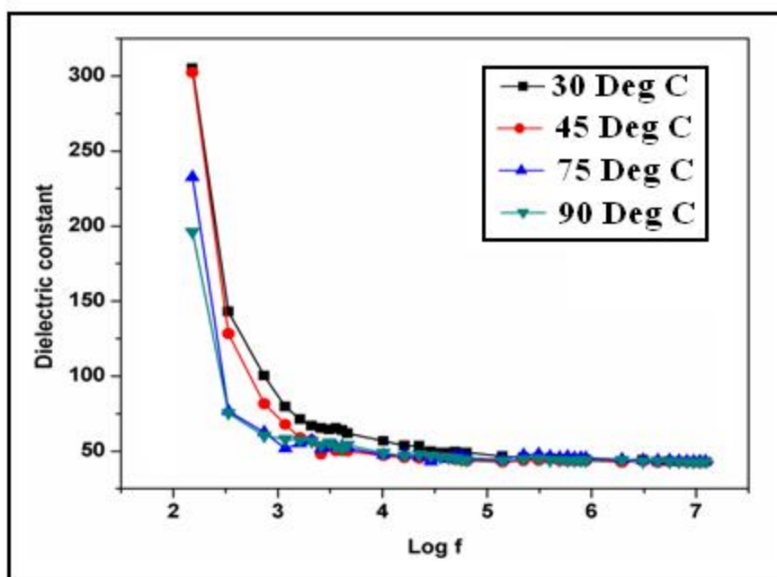
Fig.3 Variation of the dielectric constant against log f
