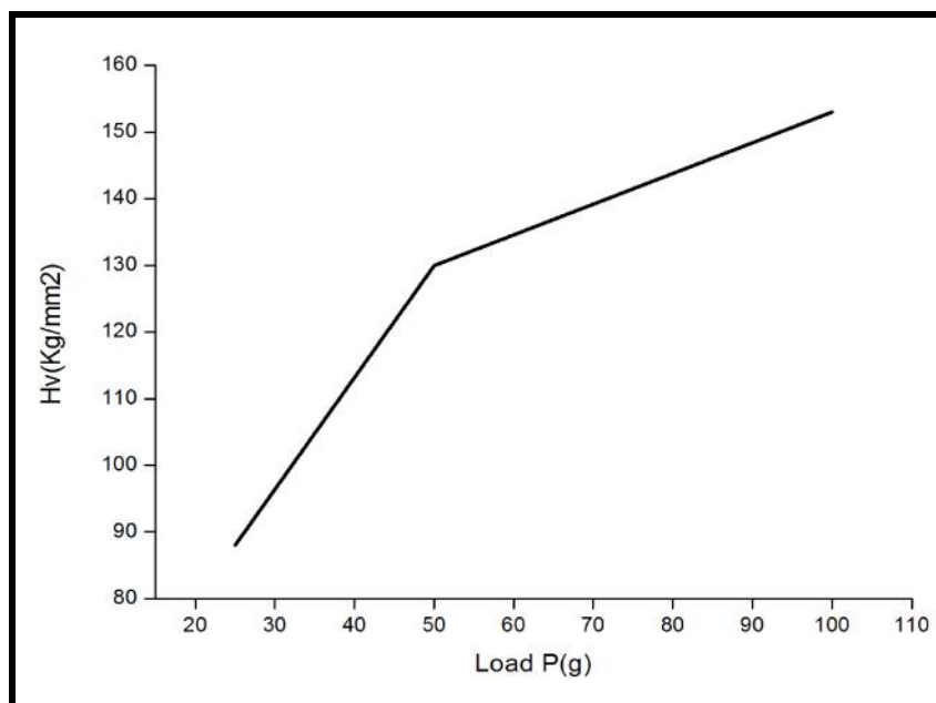
100 101 Fig.1 Variation of hardness number ( H_V ) with load P
