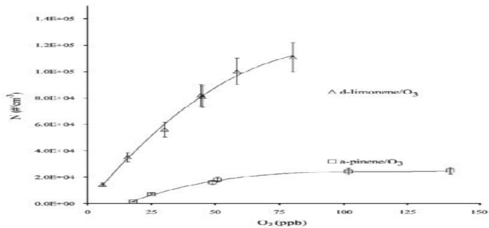
Figure 1: Effect of \text{O}_3 concentration on particle concentration Source:Nøjgaard et al. [46]
