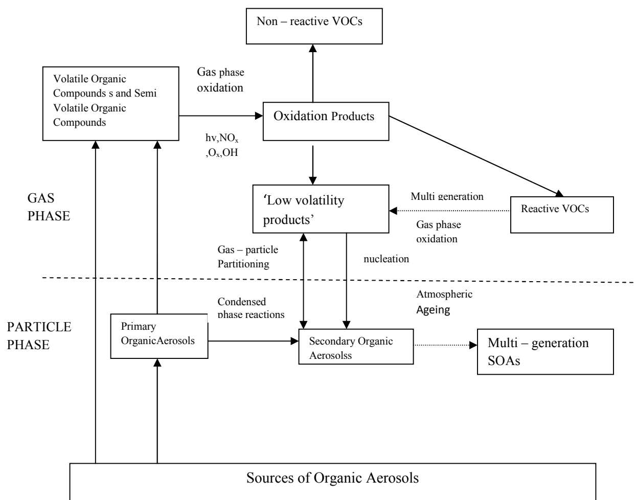
Figure 2 : Route of Formation of Secondary Organic Aerosols Source: Wang (2011) [11]
