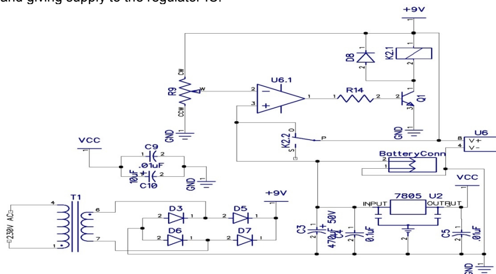
154 Fig. 5.Regulated Power Supply and Filter Circuit
