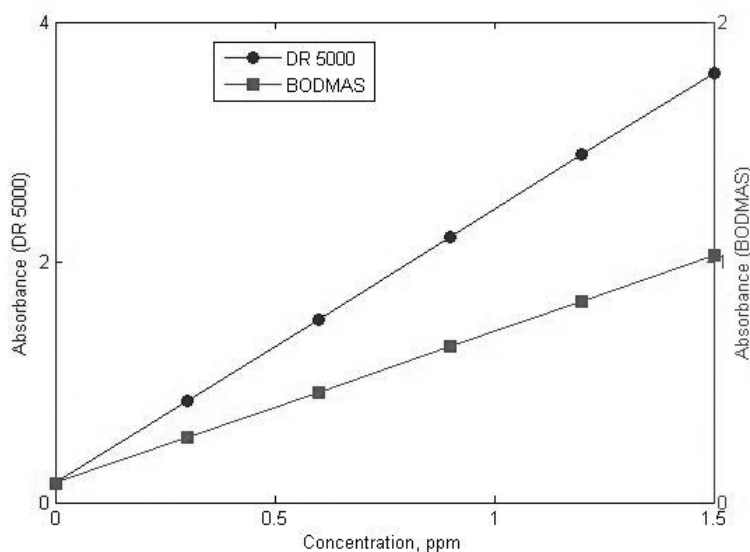
Fig. 10. Calibration characteristic
