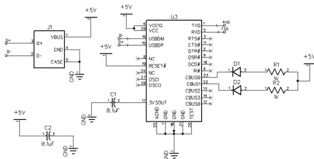
Fig. 7. Serial Communication Circuit
