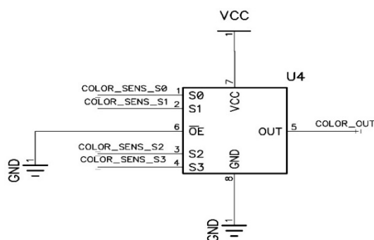
Fig. 3. Colour Sensor
