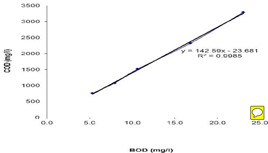
Fig. 3. COD-BOD 5 curve for Nigeria Bottling Company (NBC (Coca-Cola)) wastewater
