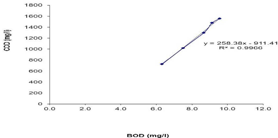
Fig. 4. COD-BOD 5 curve for Nasco Foods Ltd. (NF) wastewater
