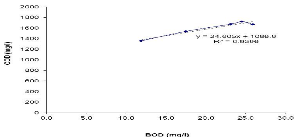
Fig. 1. COD-BOD 5 curve for Nasco Household Products Ltd. (NHPL) wastewater
